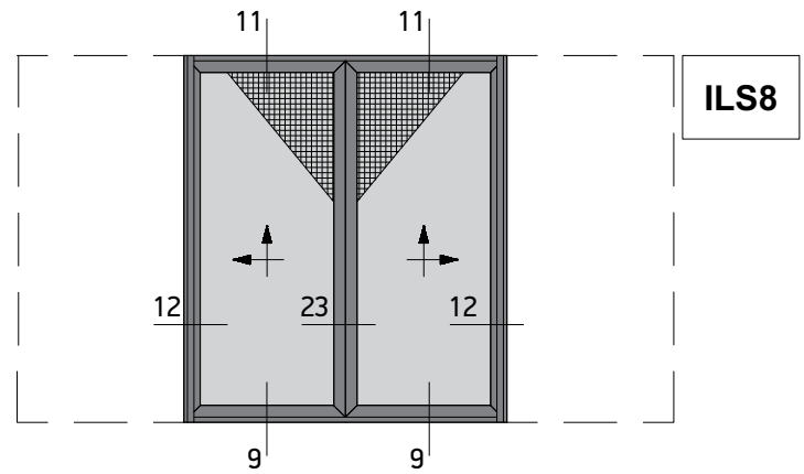
Pocket Lift@Slide Window with Meeting Stile and Narrow Flyscreen
