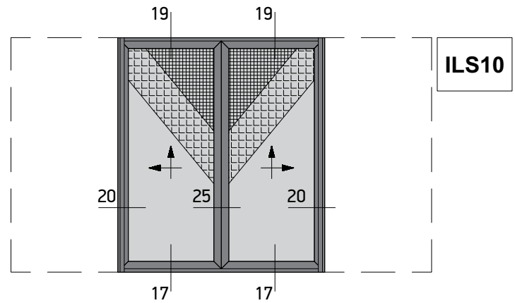
Pocket Lift@Slide Window with Meeting Stile, with Narrow Flyscreen and Shutter
