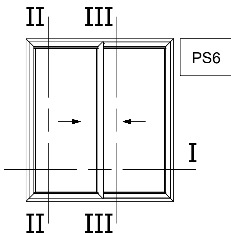
Two Sash Sliding Window 45° Cut (Sash M4542) Right
