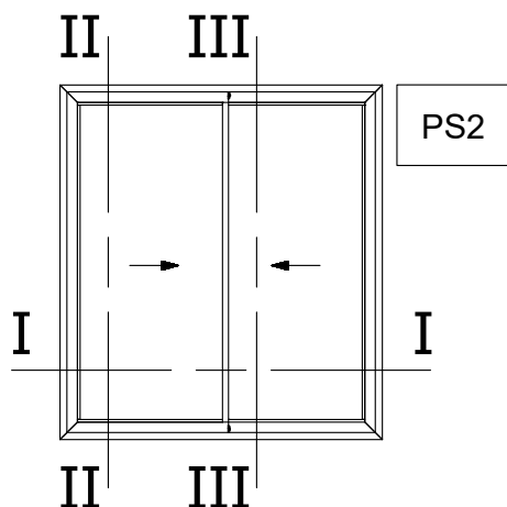
Two Sash Sliding Window 90° Cut Right
